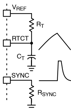
Figure 49. SYNC Pulse
