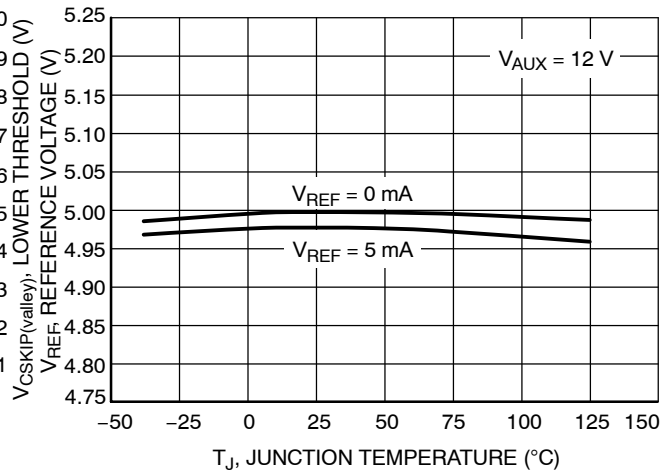
Figure 21. Reference Voltage vs. Junction Temperature
